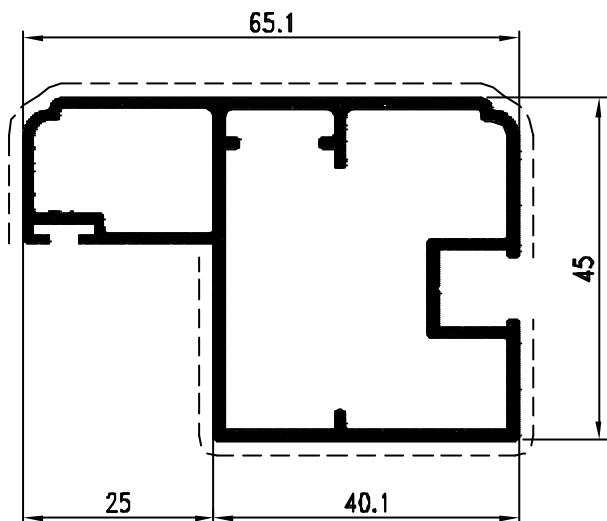
Pr. 31926 kg/m. 1.007 sup. in vista mm. 183
