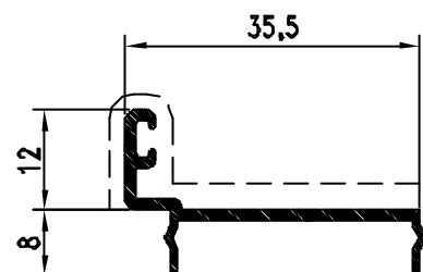
Pr. 50037 kg/m. 0.213 sup. in vista mm. 61
