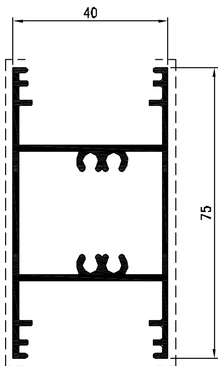
Pr. 16013 kg/m. 1.207 sup. in vista mm. 165
