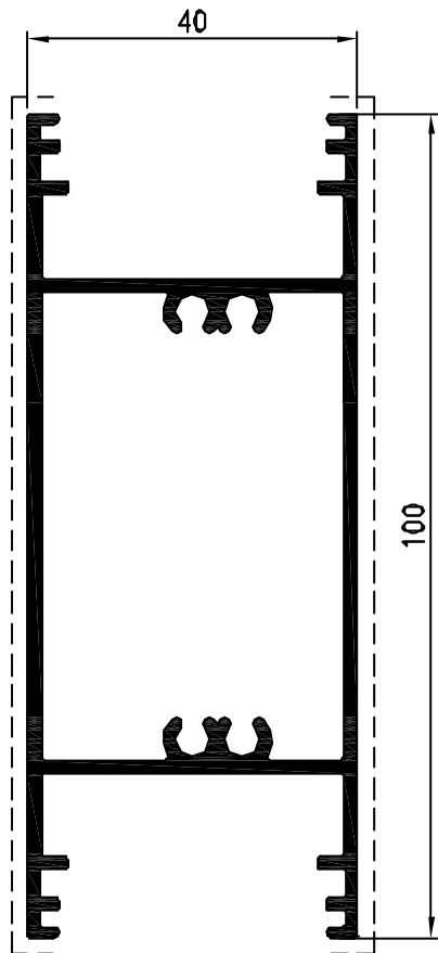
Pr. 16012 kg/m. 1.509 sup. in vista mm. 221
