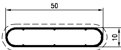
Pr. 50013 kg/m. 0.240 sup. in vista mm. 111
