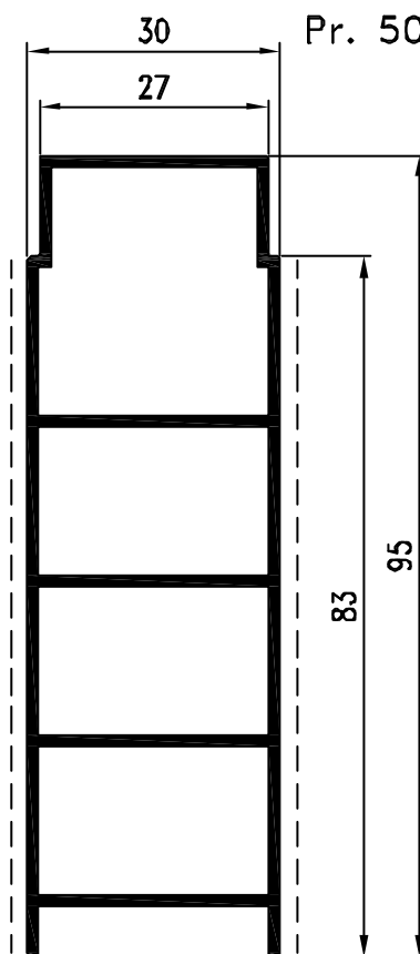
Pr. 50018 kg/m. 1.126 sup. in vista mm. 186
