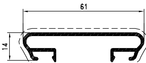
Pr. 50034 kg/m. 0.497 sup. in vista mm. 94
