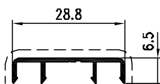
Pr. 50011 kg/m. 0.132 sup. in vista mm. 41
