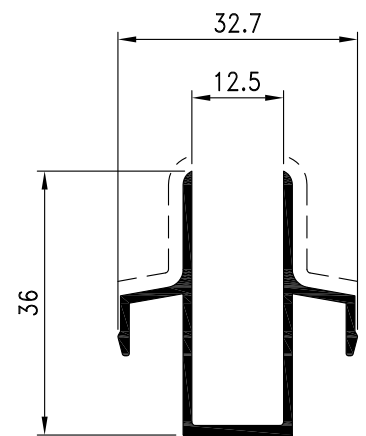
Pr. 27370 kg/m. 0.381 sup. in vista mm. 47
