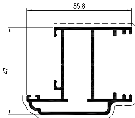
Pr. 26240 kg/m. 0.964 sup. in vista mm. 116
