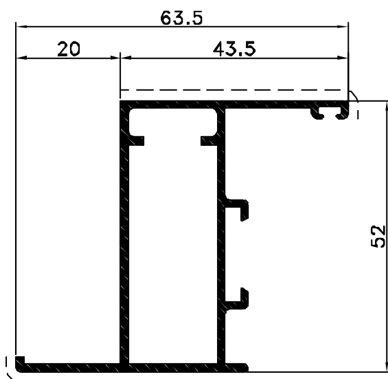
Pr. 50002 kg/m. 0.845 sup. in vista mm. 95
