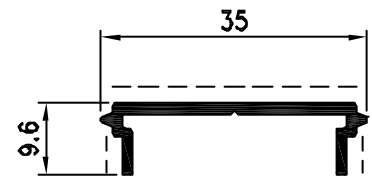
Pr. 26237 kg/m. 0.208 sup. in vista mm. 42
