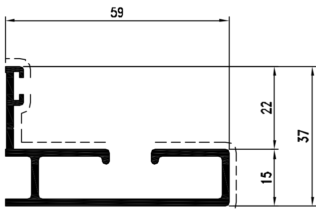
Pr. 16075 kg/m. 0.788 sup. in vista mm. 152
