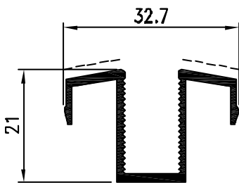
Pr. 19647 kg/m. 0.311 sup. in vista mm. 21
