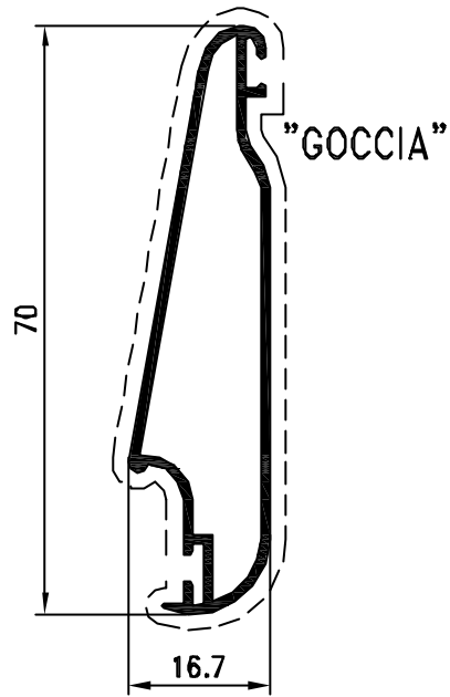
Pr. 27367 kg/m. 0.499 sup. in vista mm. 160
