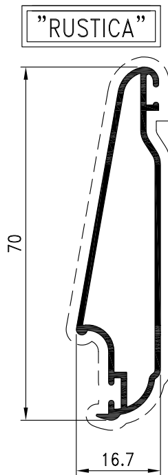
Pr. 27368 kg/m. 0.494 sup. in vista mm. 158
