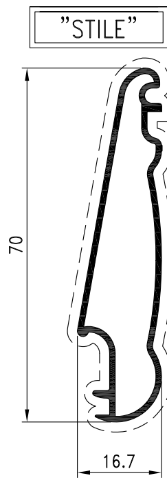
3260063 kg/m. 0.501 sup. in vista mm. 177
