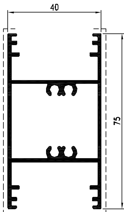
Pr. 16013 kg/m. 1.207 sup. in vista mm. 165
