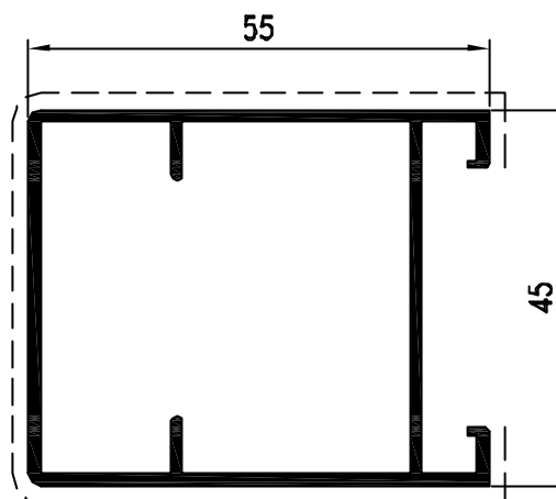
Pr. 50009 kg/m. 0.832 sup. in vista mm. 169
