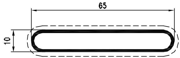
Pr. 13199 kg/m. 0.448 sup. in vista mm. 141
