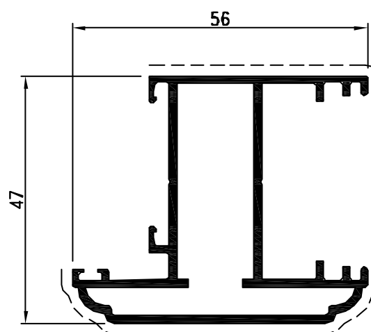
Pr 26236 Kg/m 0.994 sup. in vista mm. 116
