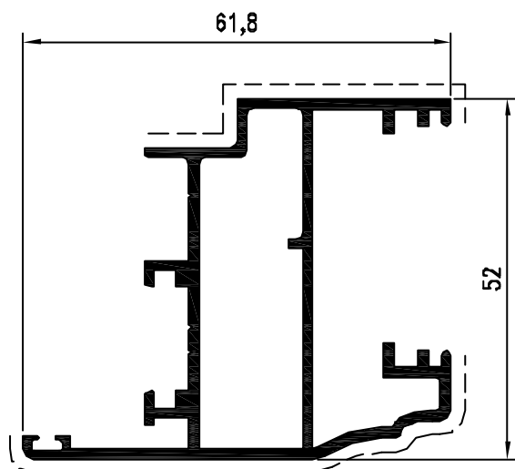
Pr 26217 Kg/m 1.040 sup. in vista mm. 129
