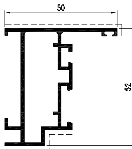
Pr. 19715 kg/m. 0.853 sup. in vista mm. 80
