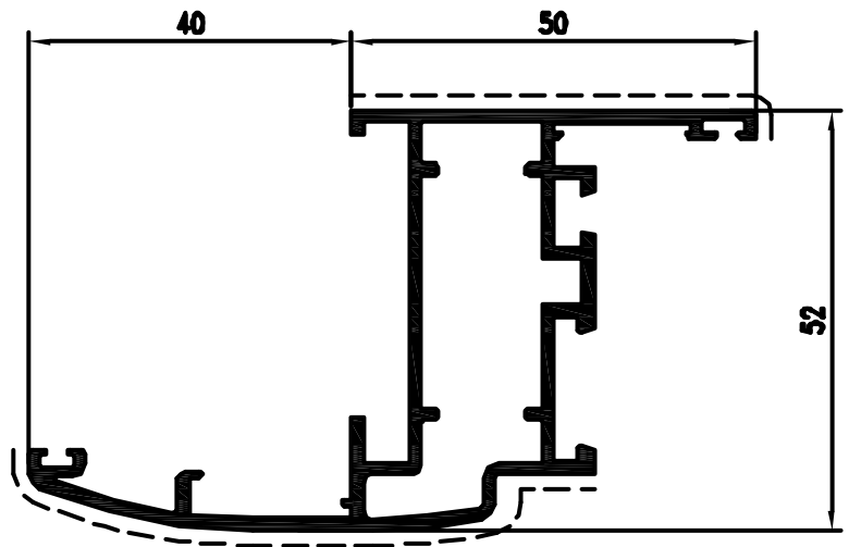
Pr. 60058 kg/m. 1.098 sup. in vista mm. 133
