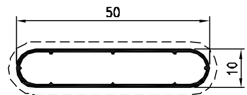
Pr. 50013 kg/m. 0.240 sup. in vista mm. 111
