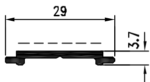
Pr. 19730 kg/m. 0.165 sup. in vista mm. 23
