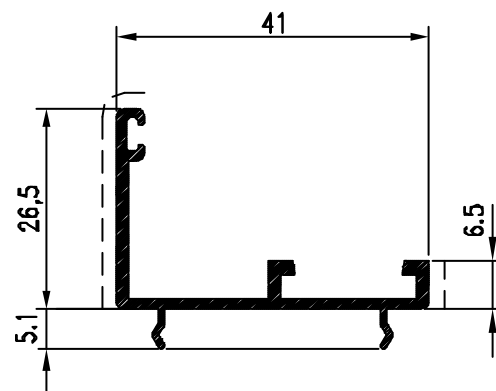
Pr. 50040 kg/m. 0.365 sup. in vista mm. 37
