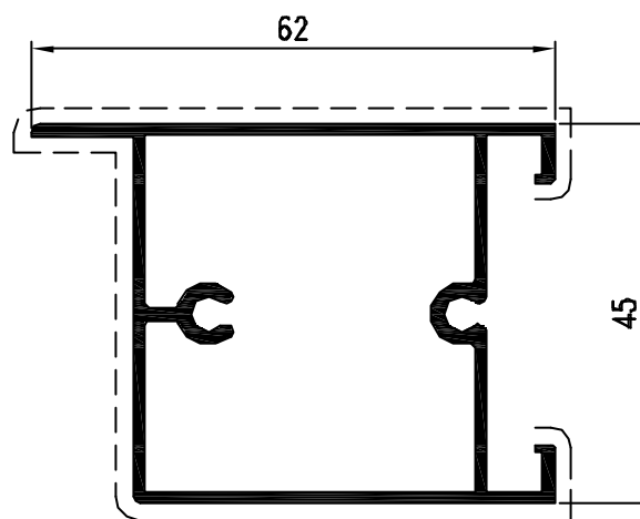
Pr. 50024 kg/m. 0.918 sup. in vista mm. 187
