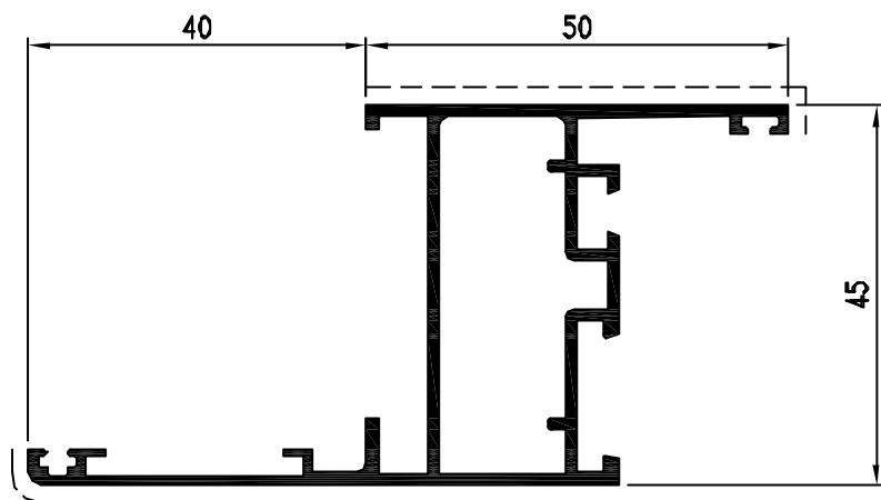
Pr. 21676 kg/m. 0.960 sup. in vista mm. 127
