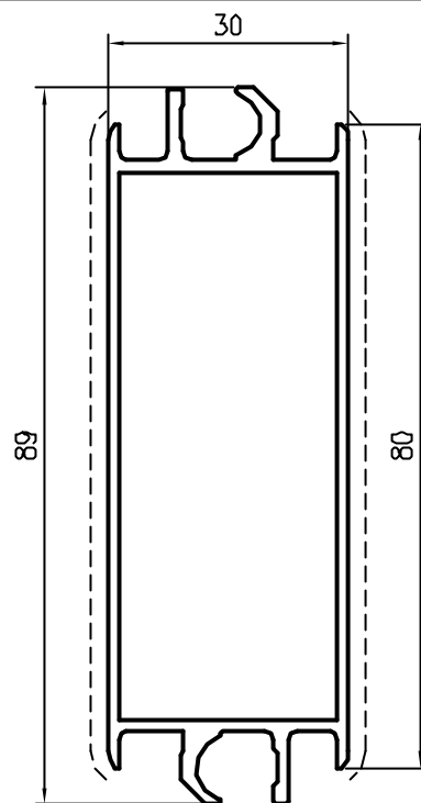
Pr 27383 kg/m. 1,015 sup.in vista mm. 160
