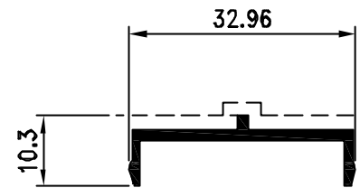
Pr. 19646 kg/m. 0.201 sup. in vista mm. 36
