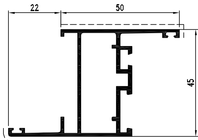
Pr. 16950 kg/m. 0.883 sup. in vista mm. 109
