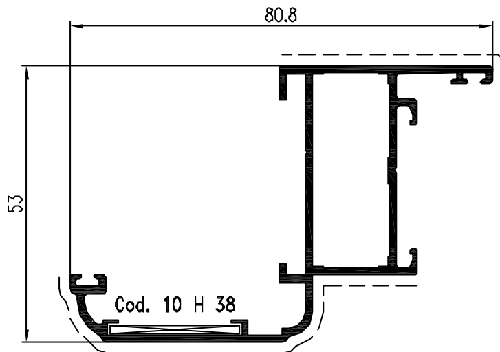
Pr. 23328 kg/m. 0.902 sup. in vista mm. 138
