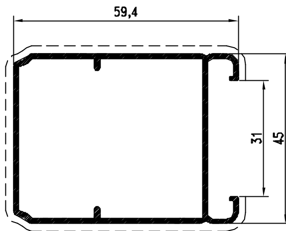
Pr. 50031 kg/m. 0.805 sup. in vista mm. 169
