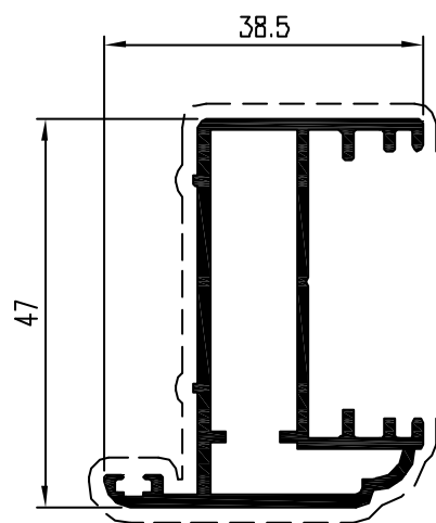
Pr. 26239 kg/m. 0.726 sup. in vista mm. 137
