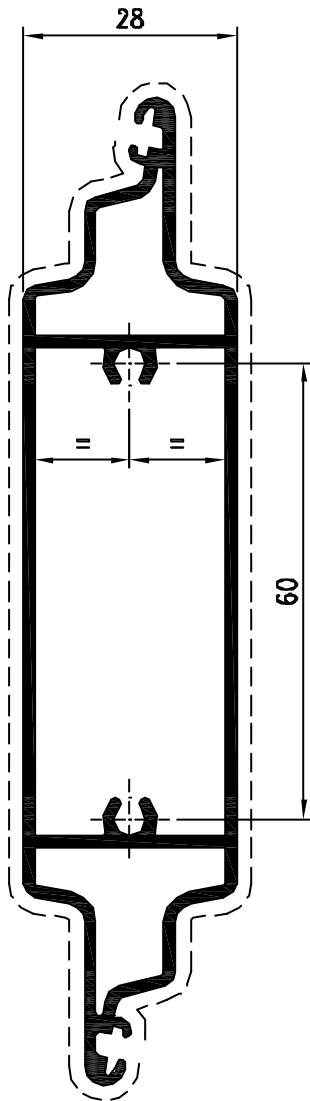
Pr. 27374 kg/m. 1.492 sup. in vista mm. 293
