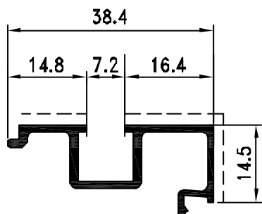
Pr. 26187 kg/m. 0.327 sup. in vista mm. 44
