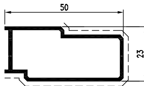
Pr. 26225 kg/m. 0.526 sup. in vista mm. 99
