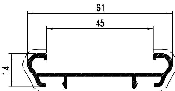
Pr. 50017 kg/m. 0.432 sup. in vista mm. 49
