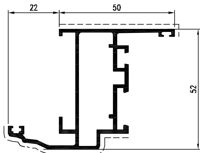
Pr. 23237 kg/m. 0.991 sup. in vista mm. 117
