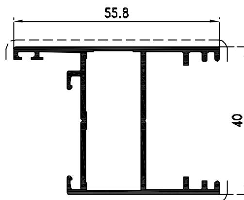
Pr 19724 Kg/m 0.748 sup. in vista mm. 108
