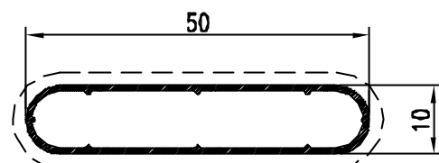
Pr. 50013 kg/m. 0.240 sup. in vista mm. 111
