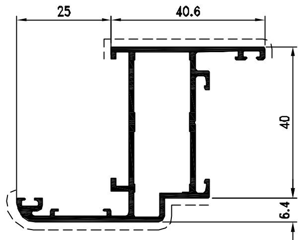
Pr 23342 Kg/m 0.805 sup. in vista mm. 104
