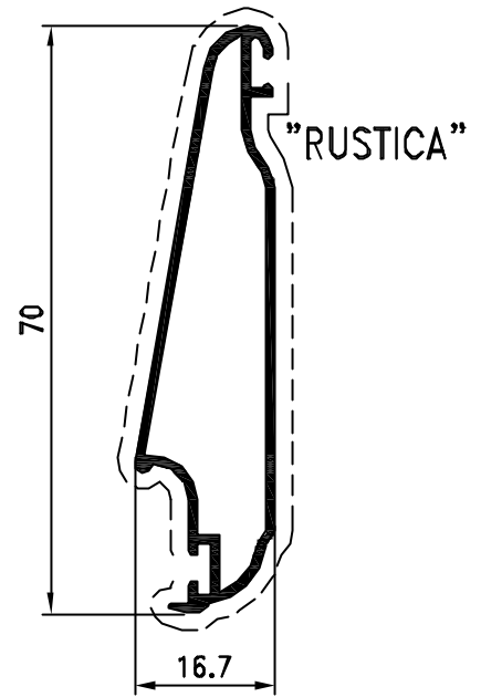
Pr. 27368 kg/m. 0.494 sup. in vista mm. 158
