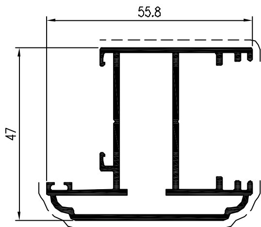
Pr. 26236 kg/m. 0.994 sup. in vista mm. 116
