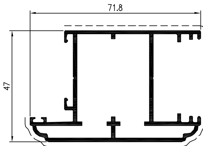
Pr. 26235 kg/m. 1.188 sup. in vista mm. 148
