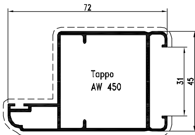
Pr. 50044 kg/m. 0.948 sup. in vista mm. 193
