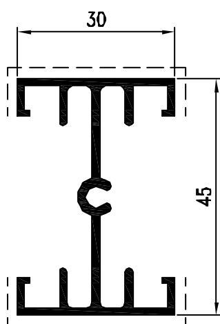
Pr. 50005 kg/m. 0.653 sup. in vista mm. 98
