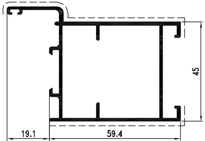
Pr. 50008 kg/m. 1.048 sup. in vista mm. 162
