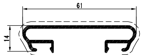
Pr. 50034 kg/m. 0.497 sup. in vista mm. 94
