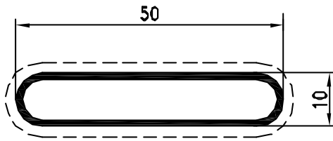
Pr. 10763 kg/m. 0.347 sup. in vista mm. 111
