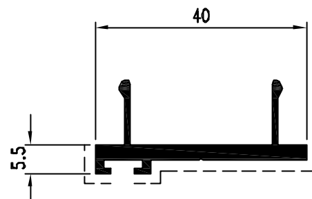
Pr. 16039 kg/m. 0.432 sup. in vista mm. 47
