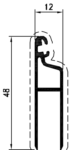
Pr. 27369 kg/m. 0.375 sup. in vista mm. 108
