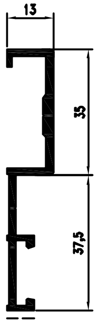
Pr. 34637 kg/m. 0.613 sup. in vista mm. 7.5
