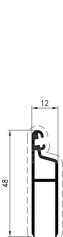
Pr. 27369 kg/m. 0.375 sup. in vista mm. 108
