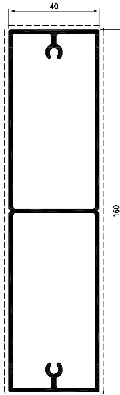
Pr. 31927 kg/m. 2.168 sup. in vista mm. 400
