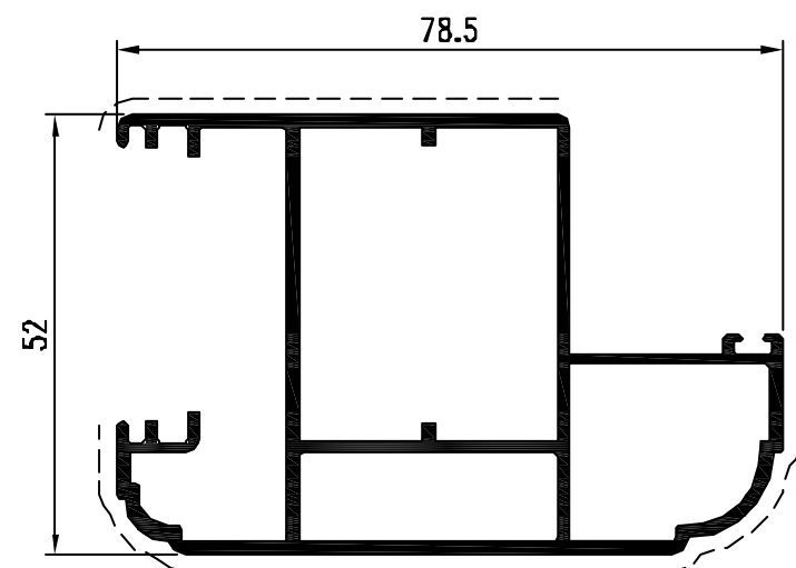
Pr. 27380 kg/m. 1.380 sup. in vista mm. 168
