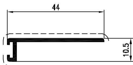
Pr. 16077 kg/m. 0.207 sup. in vista mm. 57
