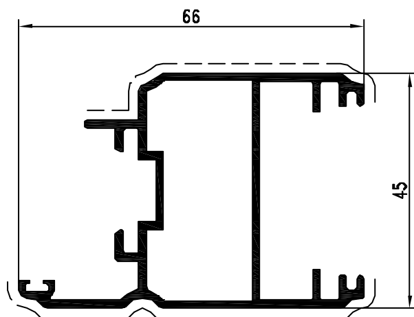
Pr. 50050 kg/m. 0.999 sup. in vista mm. 139
