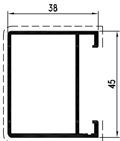
Pr. 50004 kg/m. 0.653 sup. in vista mm. 135
