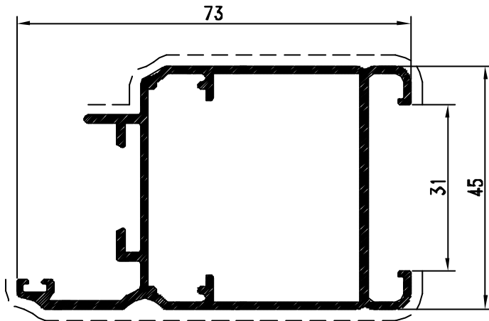
Pr. 50026 kg/m. 0.986 sup. in vista mm. 138
