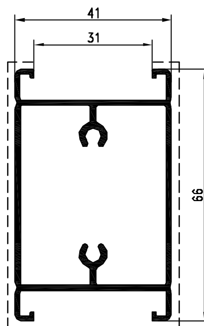
Pr. 50043 kg/m. 0.988 sup. in vista mm. 151
