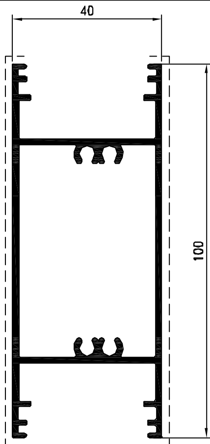
Pr. 16012 kg/m. 1.509 sup. in vista mm. 221
