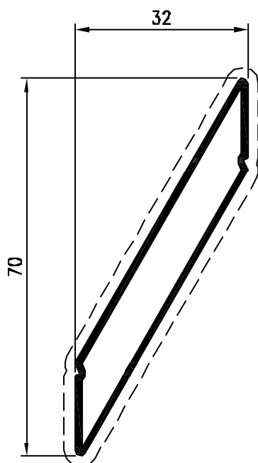
Pr. 26230 kg/m. 0.505 sup. in vista mm. 160
