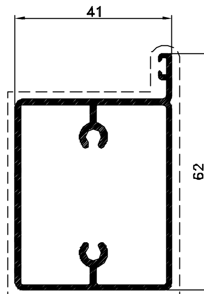
Pr. 50036 kg/m. 0.891 sup. in vista mm. 210
