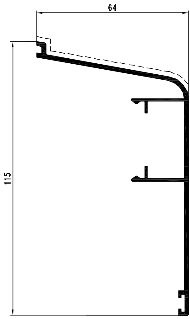
Pr. 16073 kg/m. 0.996 sup. in vista mm. 168
