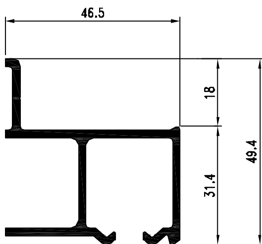
Pr. 16074 kg/m. 0.918 sup. in vista mm. =
