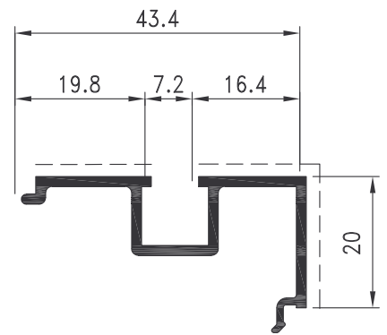
Pr. 24458 kg/m. 0.378 sup. in vista mm. 54
