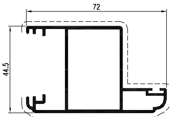
Pr. 27362 kg/m. 0.967 sup. in vista mm. 189
