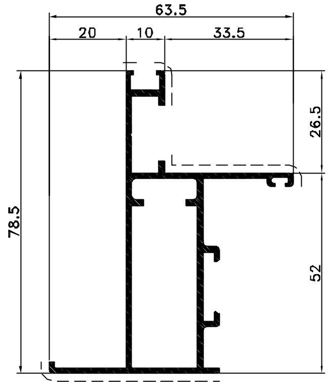
Pr. 50001 kg/m. 1.026 sup. in vista mm. 100
