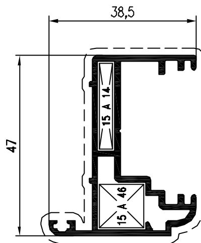
Pr. 27538 kg/m. 0.748 sup. in vista mm. 139
