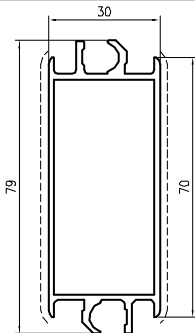
Pr 27382 kg/m. 0,940 sup.in vista mm. 140
