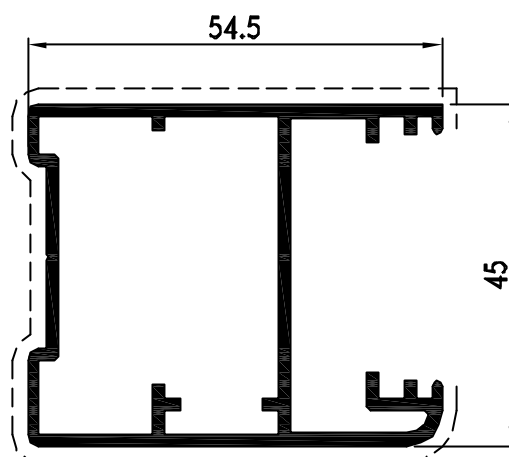
Pr. 24455 kg/m. 0.983 sup. in vista mm. 190
