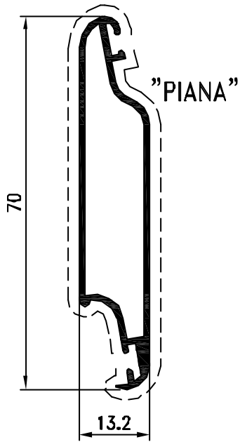
Pr. 27366 kg/m. 0.490 sup. in vista mm. 157
