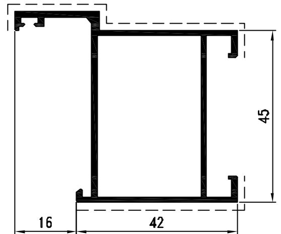
Pr. 50021 kg/m. 0.813 sup. in vista mm. 124
