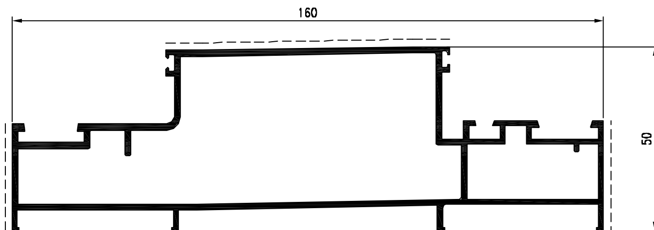
Pr. 26144 kg/m. 2.060 sup. in vista mm. 136
