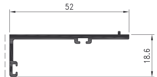
Pr. 60009 kg/m. 0.378 sup. in vista mm. 19
