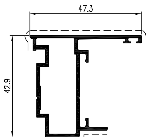
Pr. 21688 kg/m. 0.662 sup. in vista mm. 74
