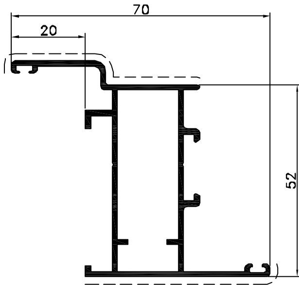
Pr. 26214 kg/m. 0.923 sup. in vista mm. 112
