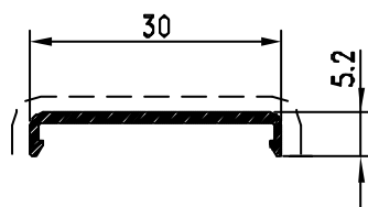
Pr. 50038 kg/m. 0.117 sup. in vista mm. 40
