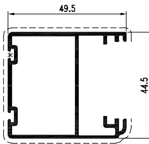
Pr. 27378 kg/m. 0.813 sup. in vista mm. 145
