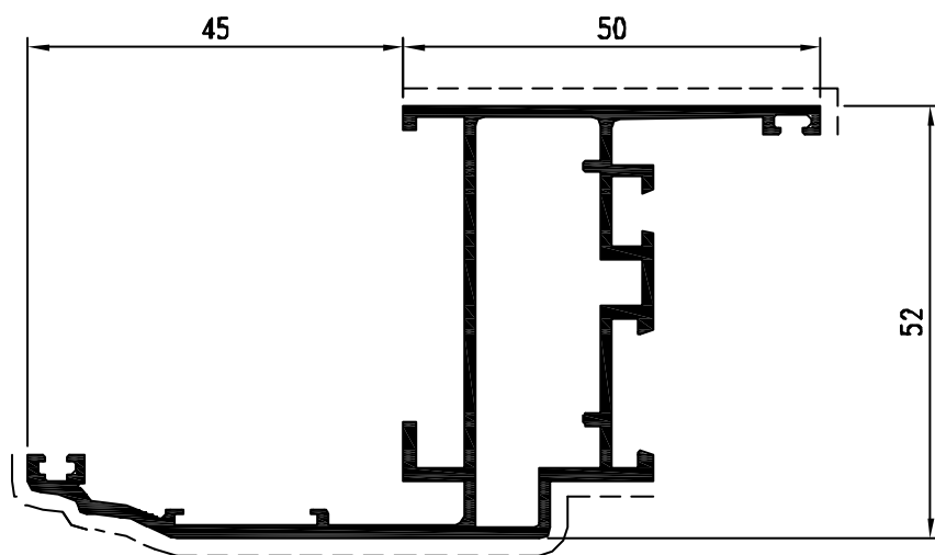
Pr. 23283 kg/m. 1.113 sup. in vista mm. 257
