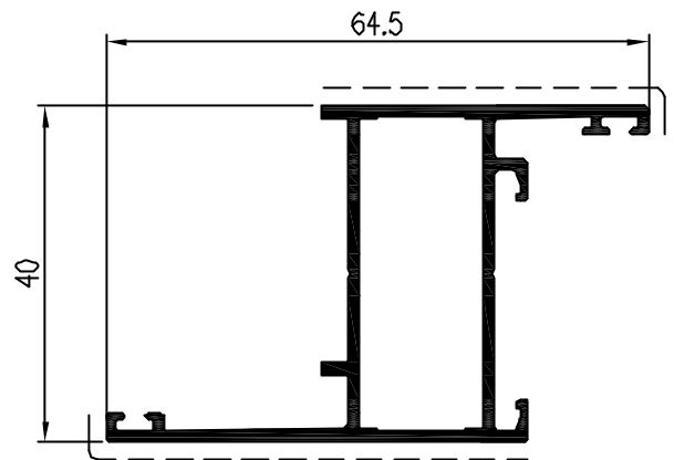
Pr. 26200 kg/m. 0.684 sup. in vista mm. 96
