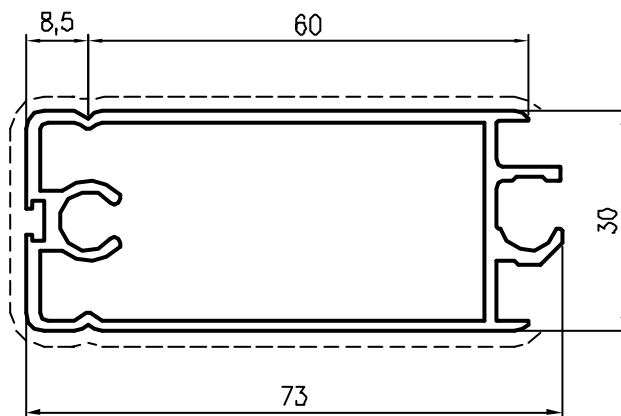
Pr 27460 kg/m. 2,014 sup.in vista mm. 348
