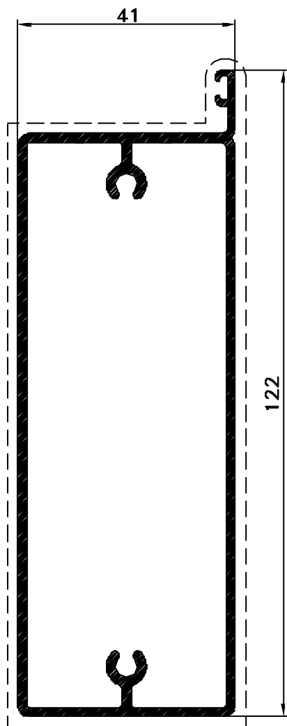
Pr. 50033 kg/m. 1.588 sup. in vista mm. 315
