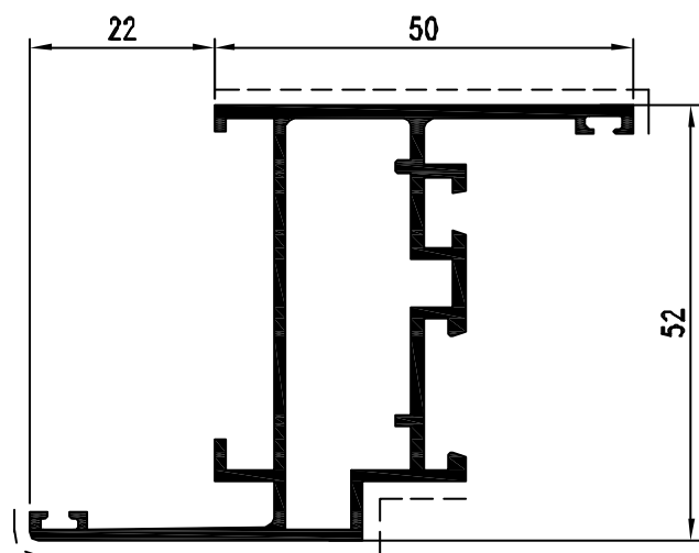
Pr. 19714 kg/m. 0.956 sup. in vista mm. 109
