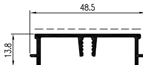
Pr. 27361 kg/m. 0.354 sup. in vista mm. 45
