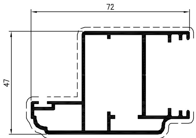
Pr. 27359 kg/m. 1.110 sup. in vista mm. 210
