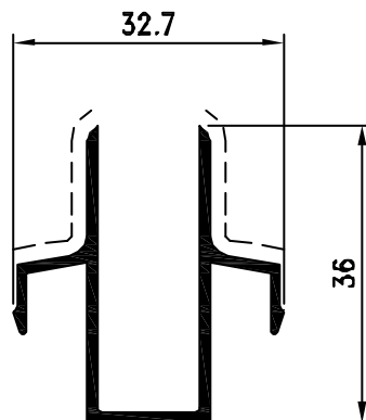
Pr. 27370 kg/m. 0.381 sup. in vista mm. 47
