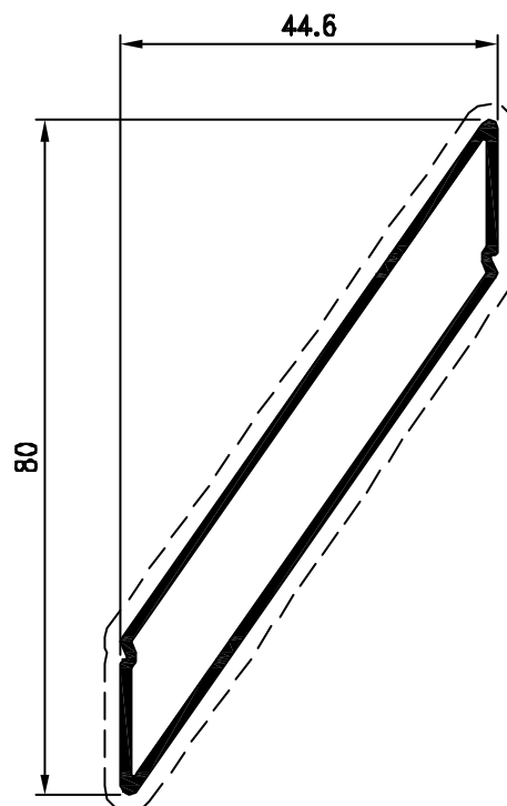
Pr. 27360 kg/m. 0.605 sup. in vista mm. 190
