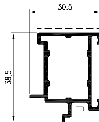
Pr. 27357 kg/mkg/m. 0.538 sup. in vista mm. 45
