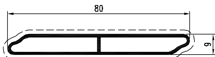
Pr. 50016 kg/m. 0.554 sup. in vista mm. 168
