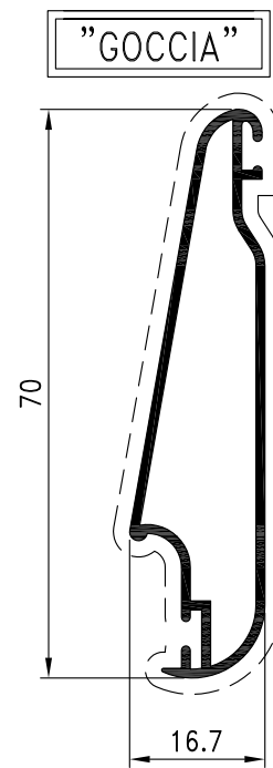
Pr. 27367 kg/m. 0.499 sup. in vista mm. 160
