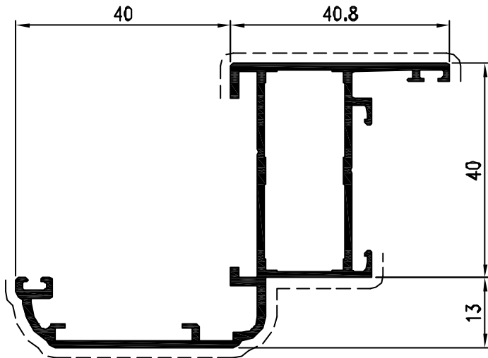
Pr 23328 Kg/m 0.902 sup. in vista mm. 138
