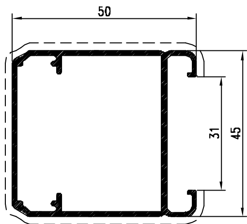
Pr. 50030 kg/m. 0.764 sup. in vista mm. 152
