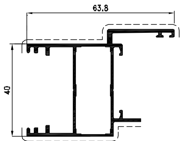
Pr 19723 Kg/m 0.853 sup. in vista mm. 137
