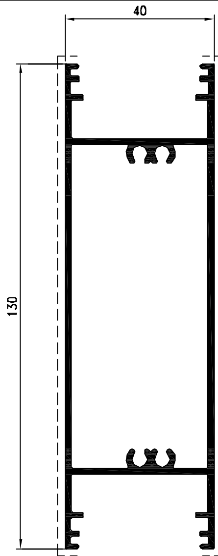
Pr. 26210 kg/m. 1.785 sup. in vista mm. 262
