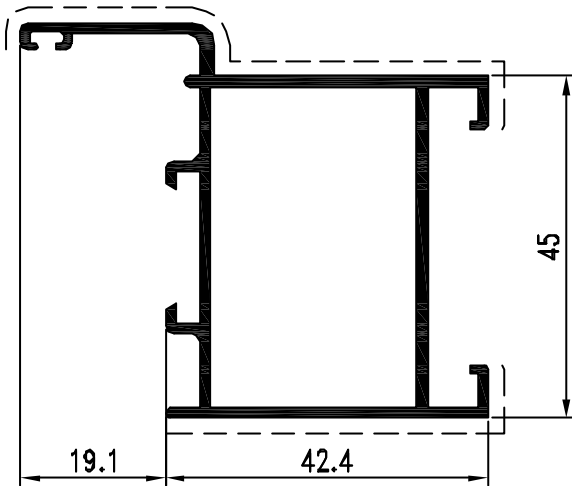
Pr. 50003 kg/m. 0.867 sup. in vista mm. 128
