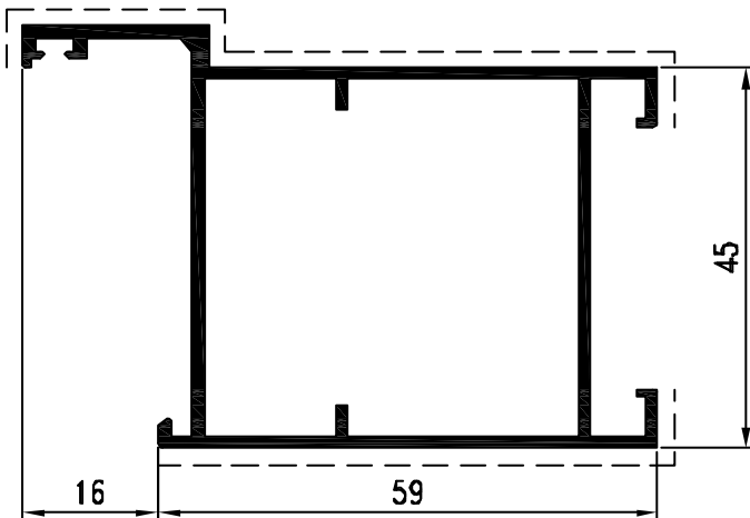
Pr. 50020 kg/m. 0.969 sup. in vista mm. 158
