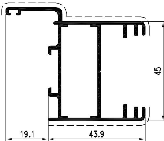
Pr. 26215 kg/m. 0.975 sup. in vista mm. 126
