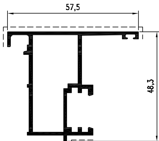
Pr. 19663 kg/m. 0.826 sup. in vista mm. 82
