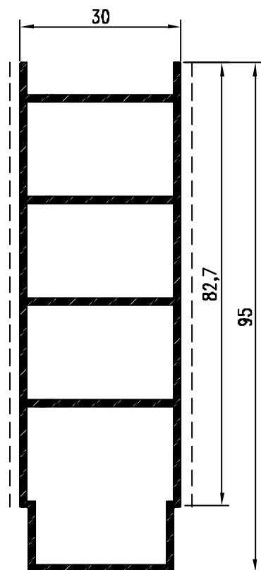
Pr. 50018 kg/m. 1.148 sup. in vista mm. 166
