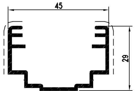
Pr. 50019 kg/m. 0.505 sup. in vista mm. 54
