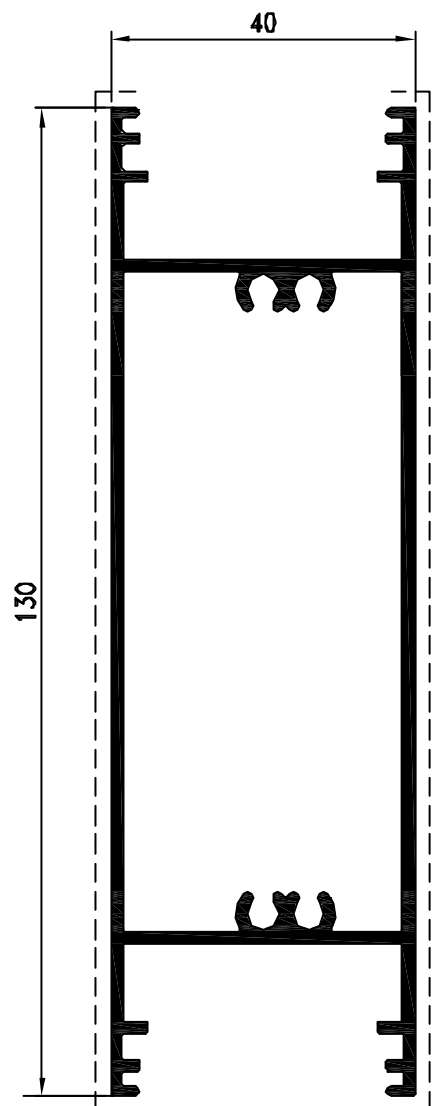
Pr. 26210 kg/m. 1.785 sup. in vista mm. 272
