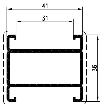
Pr. 50035 kg/m. 0.597 sup. in vista mm. 92
