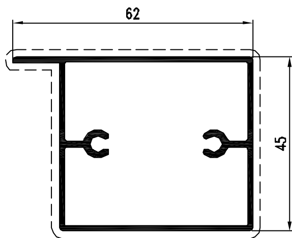
Pr. 50006 kg/m. 0.918 sup. in vista mm. 212
