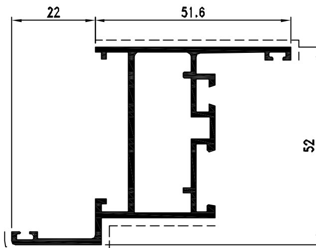
Pr. 16973 kg/m. 0.924 sup. in vista mm. 119
