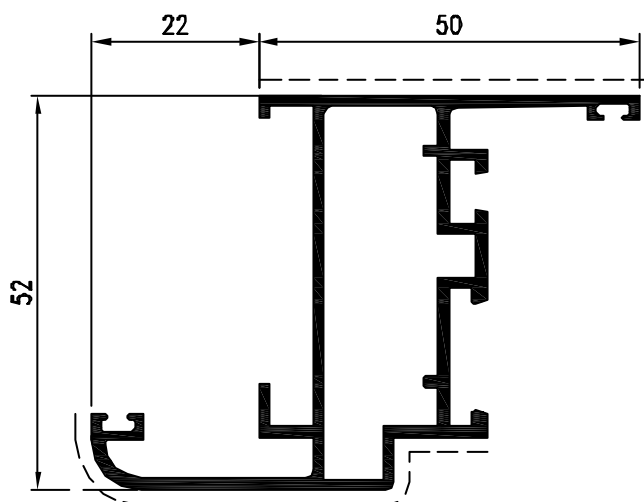
Pr. 26137 kg/m. 1.018 sup. in vista mm. 119
