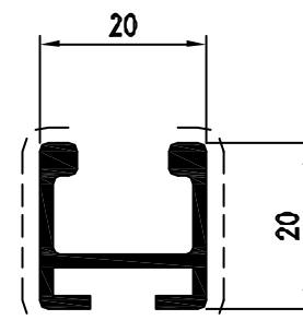
Pr. 16076 kg/m. 0.329 sup. in vista mm. 61
