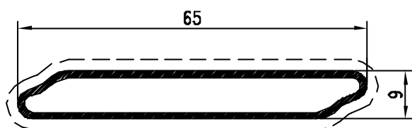
Pr. 50012 kg/m. 0.435 sup. in vista mm. 138
