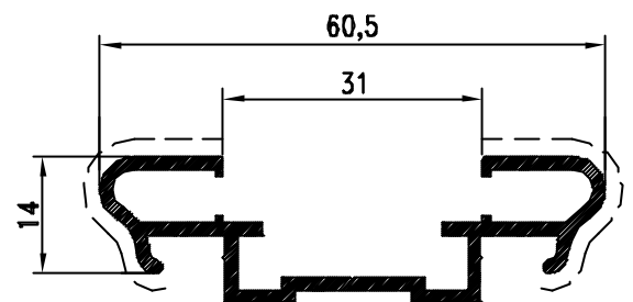
Pr. 50014 kg/m. 0.545 sup. in vista mm. 60
