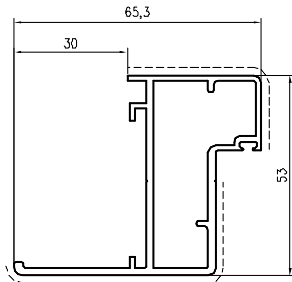
Pr 60155 kg/m. 1,040 sup.in vista mm. 140
