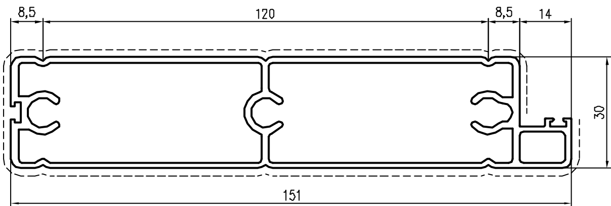
Pr 27460 kg/m. 2,014 sup.in vista mm. 348
