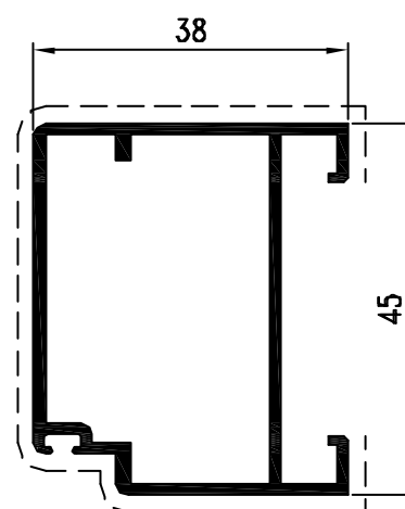
Pr. 50015 kg/m. 0.675 sup. in vista mm. 132
