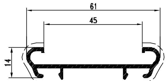
Pr. 50017 kg/m. 0.432 sup. in vista mm. 49
