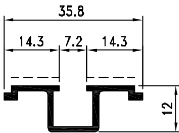
Pr. 16060 kg/m. 0.262 sup. in vista mm. 25
