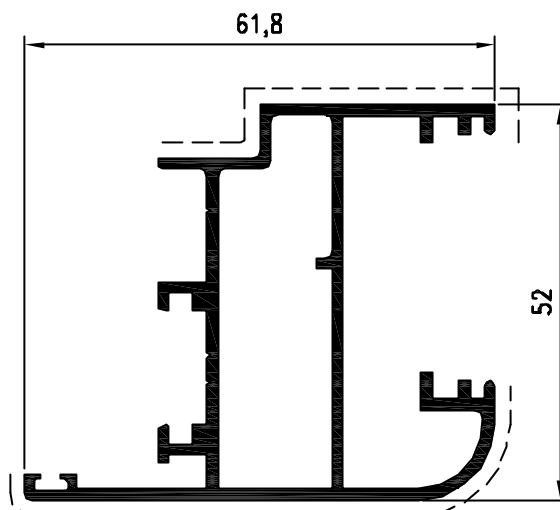
Pr. 24457 kg/m. 1.040 sup. in vista mm. 130
