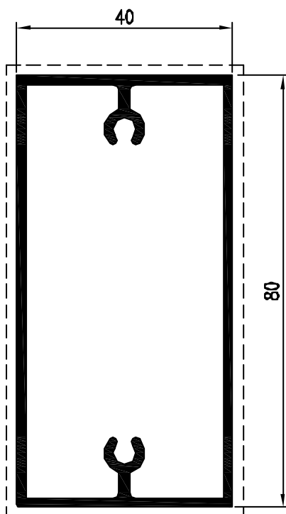
Pr. 03361 kg/m. 1.277 sup. in vista mm. 240
