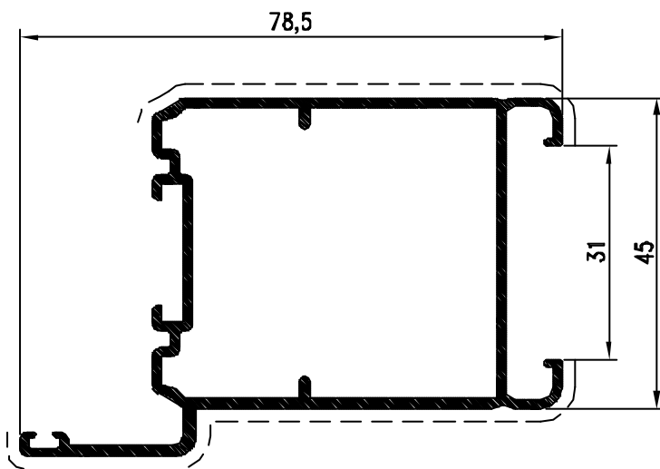
Pr. 50028 kg/m. 0.993 sup. in vista mm. 151
