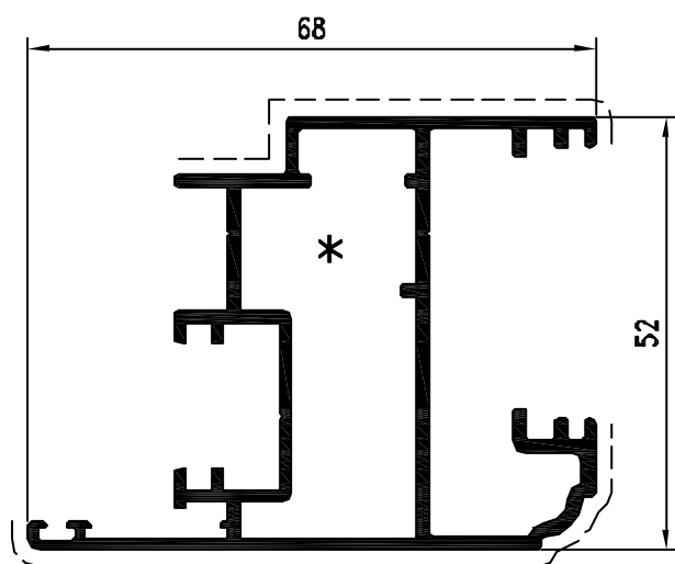
Pr 27394 Kg/m 1.153 sup. in vista mm. 142
