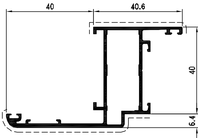
Pr 23341 Kg/m 0.894 sup. in vista mm. 119
