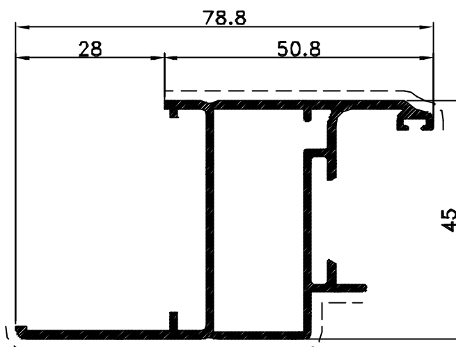
Pr. 50025 kg/m. 0.905 sup. in vista mm. 134
