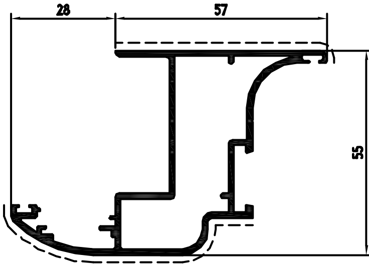
Pr. 34636 kg/m. 1.131 sup. in vista mm. 138
