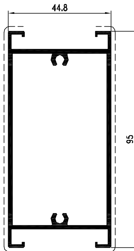
Pr. 50039 kg/m. 1.431 sup. in vista mm. 216
