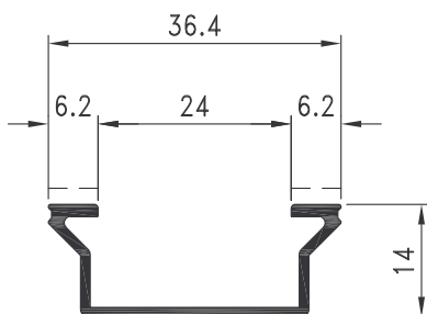
Pr. 60396 kg/m. 0.227 sup. in vista mm. 12
