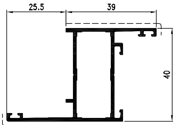
Pr 26200 Kg/m 0.684 sup. in vista mm. 96
