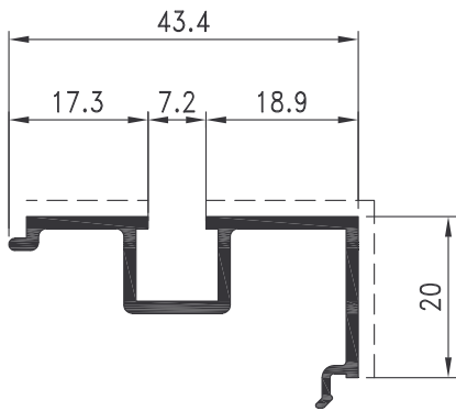
Pr. 24456 kg/m. 0.378 sup. in vista mm. 54
