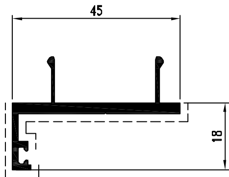
Pr. 16038 kg/m. 0.537 sup. in vista mm. 81
