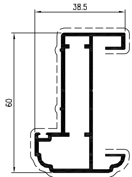
Pr. 26238 kg/m. 0.840 sup. in vista mm. 161
