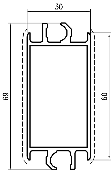
Pr 27381 kg/m. 0,864 sup.in vista mm. 120
