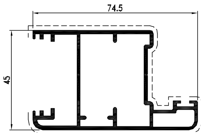
Pr. 24451 kg/m. 1.208 sup. in vista mm. 210
