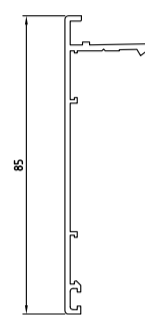
D3074009 kg/m. 0.517 sup. in vista mm. 94 CLIP D4280027
