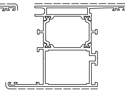
D1220064 kg/m. 1.887 sup. in vista mm. 155
