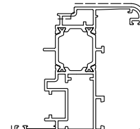
D1211009 kg/m. 1.612 sup. in vista mm. 116
