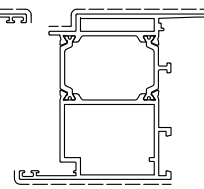
D1220070 kg/m. 1.717 sup. in vista mm. 147.5
