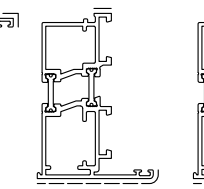
D1211032 kg/m. 1.329 sup. in vista mm. 57
