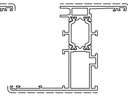
D1211018 kg/m. 1.474 sup. in vista mm. 129
