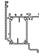
D1210859 Kg/m 1.935 Sup. in vista mm 168
