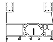
D1074004 kg/m. 1.662 sup. in vista mm. 184
