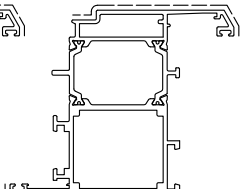
D1211023 kg/m. 1.987 sup. in vista mm. 150
