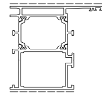
D1220065 kg/m. 1.773 sup. in vista mm. 130
