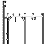
D1210862 Kg/m 1.792 Sup. in vista mm 145
