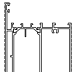
D1210860 Kg/m 2.702 Sup. in vista mm 225
