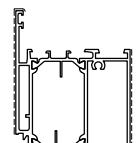
D1210859 Kg/m 1.935 Sup. in vista mm 168
