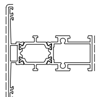
D1211007 kg/m. 1.433 sup. in vista mm. 109
