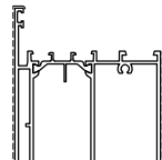
D1210857 Kg/m 2.018 Sup. in vista mm 168
