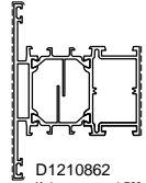
D1210862 Kg/m 1.732 Sup. in vista mm 145
