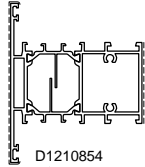
D1210854 Kg/m 1.967 Sup. in vista mm 145
