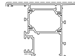
D1220073 kg/m. 2.130 sup. in vista mm. 175
