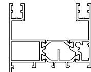
D1074003 kg/m. 1.649 sup. in vista mm. 167
