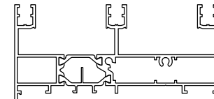
D1074005 kg/m. 2.447 sup. in vista mm. 199
