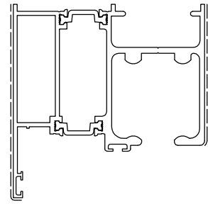
D1250007 Kg/m 2.560 Sup. in vista mm 146
