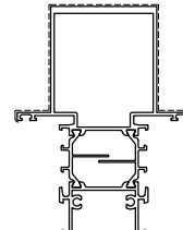
D1210870 Kg/m 2.736 Sup. in vista mm 255
