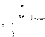
D3074008 kg/m. 0.549 sup. in vista mm. 84 CLIP D4280027
