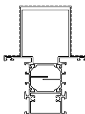
D1210870 Kg/m 2.736 Sup. in vista mm 255
