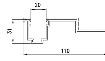
D3290150 sup.vista mm. 122.8 Kg./m 0.993
