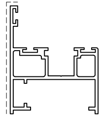
D3250004 kg/m 1.024 sup. in vista mm 98
