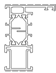
D1210762 Kg/m 1.263 Sup. in vista mm 82
