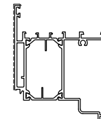
D1210857 Kg/m 2.018 Sup. in vista mm 168
