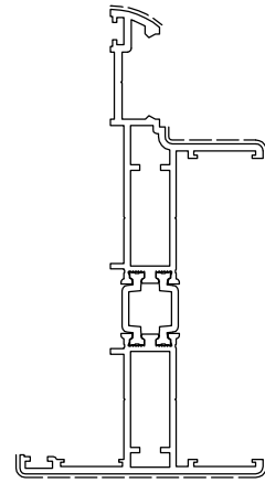
D1250014 Kg/m 2.081 Sup. in vista mm 123
