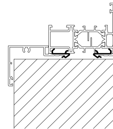
D3074008 kg/m. 0.549 sup. in vista mm. 84 CLIP D4280027
