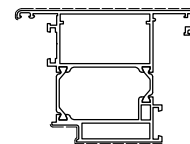
D1210888 Kg/m 2.390 Sup. in vista mm 193
