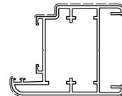
D3220093 Kg/m 1.248 Sup. in vista mm 140
