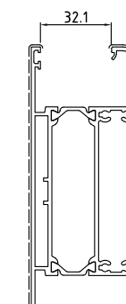
D1210456 Kg/m 2.644 Sup. in vista mm 287
