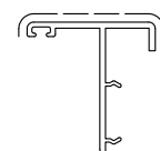
D0050110 kg/m. 0.292 Sup. in vista 49
