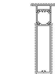
D1211027 Kg/m 2.060 Sup. in vista mm 261
