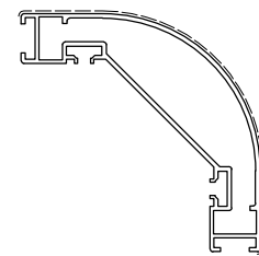
D0027480 Kg/m 1.59 Sup. in vista mm 157
