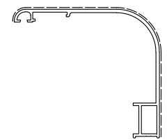
D3220110 Kg/m 0.984 Sup. in vista mm 152
