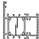
D1210863 Kg/m 1.865 Sup. in vista mm 145
