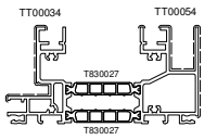
T141000 Kg/m 2.1970 Sup. in vista mm 188
