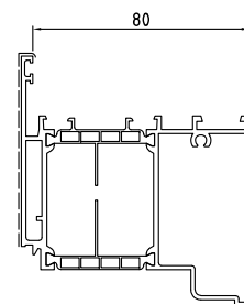
D1060045 Kg/m 2.101 Sup. in vista mm 144
