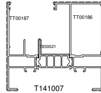
T141007 Kg/m 2.4780 Sup. in vista mm 273
