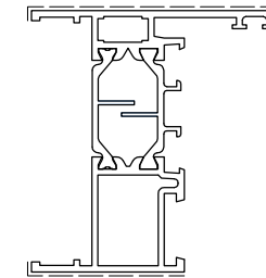
D1057006 Kg/m 1.281 Sup. in vista mm 131
