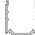
D0027479 Kg/m 0.948 Sup. in vista mm 95
