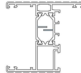
D1057005 Kg/m 1.448 Sup. in vista mm 161
