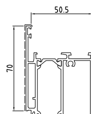
D1210459 Kg/m 1.858 Sup. in vista mm 144
