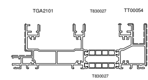
TGA1101 Kg/m 3.002 Sup. in vista mm 204
