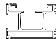
D0027462 Kg/m 1.952 Sup. in vista mm 103
