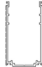
D0027478 Kg/m 1.326 Sup. in vista mm 165
