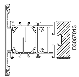
D1057055 Kg/m 1.884 Sup. in vista mm 99
