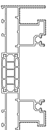
SC9K027 sup. vista mm. 383 Kg./m 3.936
