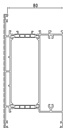
D1060056 Kg/m 3.425 Sup. in vista mm 311
