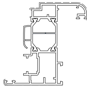
D1057022 Kg/m 1.646 Sup. in vista mm 179
