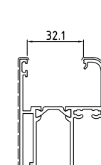
D1210455 Kg/m 1.634 Sup. in vista mm 153
