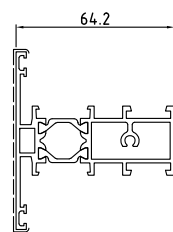
D1210453 Kg/m 1.473 Sup. in vista mm 109
