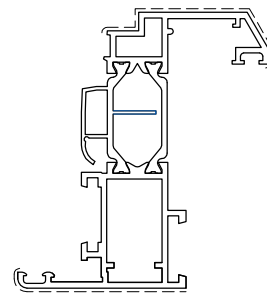
D1057013 Kg/m 1.419 Sup. in vista mm 164
