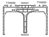
T141019 Kg/m 2.045 Sup. in vista mm 243
