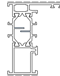
D1057004 Kg/m 1.197 Sup. in vista mm 82
