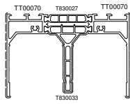
T141017 Kg/m 1.97 Sup. in vista mm 141
