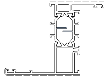
D1057002 Kg/m 1.417 Sup. in vista mm 126
