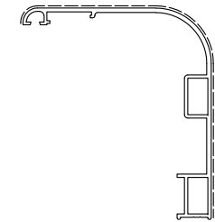
D3220111 Kg/m 1.215 Sup. in vista mm 172
