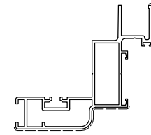
D0027484 Kg/m 1.385 Sup. in vista mm 103
