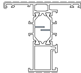
D1057001 Kg/m 1.331 Sup. in vista mm 110
