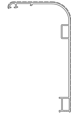
D3220141 Kg/m 1.538 Sup. in vista mm 536
