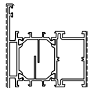
D1210862 Kg/m 1.792 Sup. in vista mm 145
