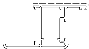
D0050101 kg/m. 0.778 Sup. in vista 109
