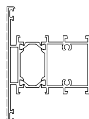
D1210454 Kg/m 1.837 Sup. in vista mm 145
