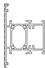
D1210463 Kg/m 1.749 Sup. in vista mm 145
