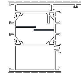
D1057007 Kg/m 1.641 Sup. in vista mm 131
