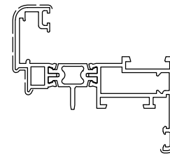
D1061002 Kg/m 1.168 Sup. in vista mm 97
