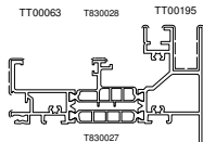
T141029 Kg/m 2.0350 Sup. in vista mm 171
