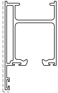
D3250003 kg/m 1.566 sup. in vista mm 146
