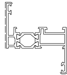
D1061001 Kg/m 1.108 Sup. in vista mm 93
