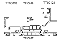
T141025 Kg/m 1.948 Sup. in vista mm 139
