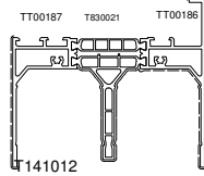
T141012 Kg/m 2.1190 Sup. in vista mm 248
