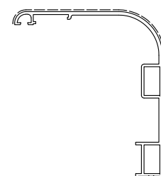
D3220111 Kg/m 1.215 Sup. in vista mm 172
