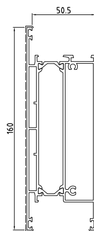
D1210468 Kg/m 3.219 Sup. in vista mm 311
