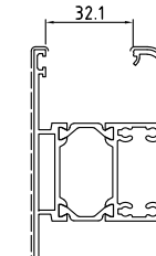
D1210458 Kg/m 1.859 Sup. in vista mm 207
