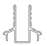
D3260267 kg/m. 0.395 sup. in vista mm. 67
