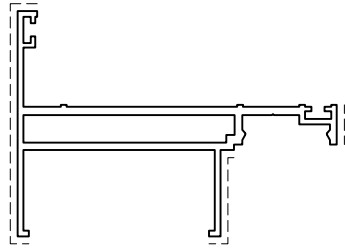
D3250002 kg/m 1.296 sup. in vista mm 108
