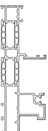
SC9K028 sup. vista mm. 255 Kg./m 3.476
