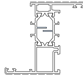
D1057003 Kg/m 1.331 Sup. in vista mm 109
