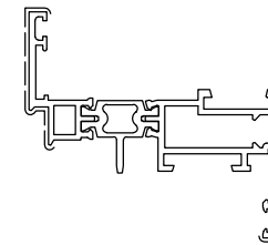
D1061004 Kg/m 1.088 Sup. in vista mm 88
