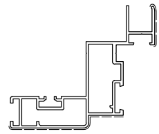
D3354005 Kg/m 1.452 Sup. in vista mm 100
