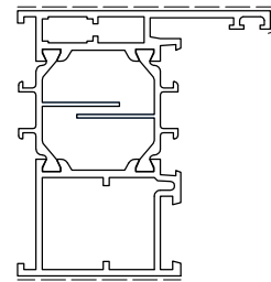
D1057000 Kg/m 1.470 Sup. in vista mm 107
