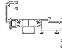
D1211282 Kg/m 1.211 Sup. in vista mm 97
