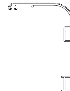
D3220112 Kg/m 1.323 Sup. in vista mm 192
