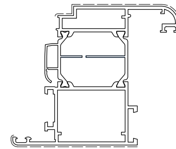
D1057014 Kg/m 1.868 Sup. in vista mm 183
