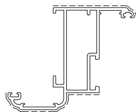
D3260255 kg/m. 0.884 sup. in vista mm. 106
