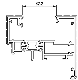
D1061006 Kg/m 1.344 Sup. in vista mm 135
