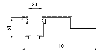
D3290150 sup.vista mm. 122.8 Kg./m 0.993
