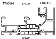
T141026 Kg/m 1.9220 Sup. in vista mm 172
