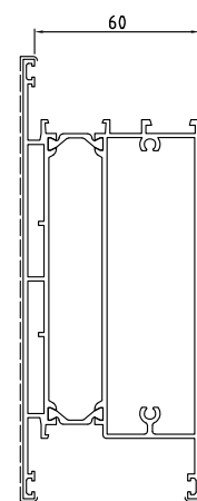
D1210469 Kg/m 3.309 Sup. in vista mm 311
