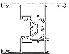
SC9V151 sup. vista mm. 169 Kg./m 2.097
