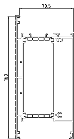
D1060055 Kg/m 3.336 Sup. in vista mm 311
