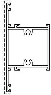
D3250021 kg/m 1.031 sup. in vista mm 133
