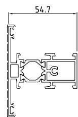
D1210452 Kg/m 1.377 Sup. in vista mm 109
