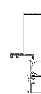
D1210470 Kg/m 2.62 Sup. in vista mm 255
