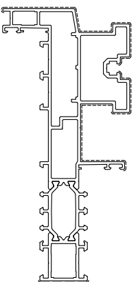
SC9K018 sup. vista mm. 273 Kg./m 3.376
