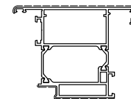
D1210890 Kg/m 2.383 Sup. in vista mm 191
