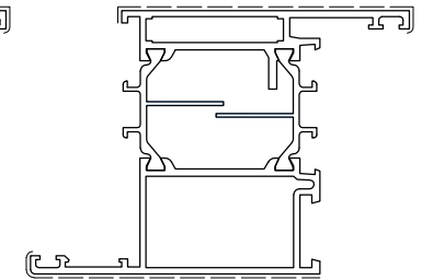
D1057008 Kg/m 1.774 Sup. in vista mm 154
