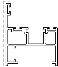
D3250004 kg/m 1.024 sup. in vista mm 98
