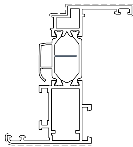
D1057010 Kg/m 1.356 Sup. in vista mm 158
