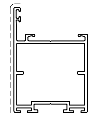
D0019656 kg/m 0.848 sup. in vista mm 105
