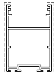
D3250012 kg/m 0.923 sup. in vista mm 126
