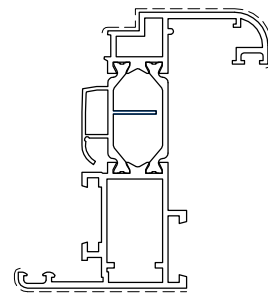
D1057012 Kg/m 1.422 Sup. in vista mm 164
