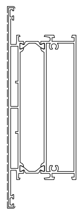
D1210467 Kg/m 3.112 Sup. in vista mm 285
