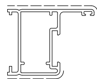
D0050100 kg/m. 0.664 Sup. in vista 82
