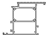
D1210880 Kg/m 2.224 Sup. in vista mm 186
